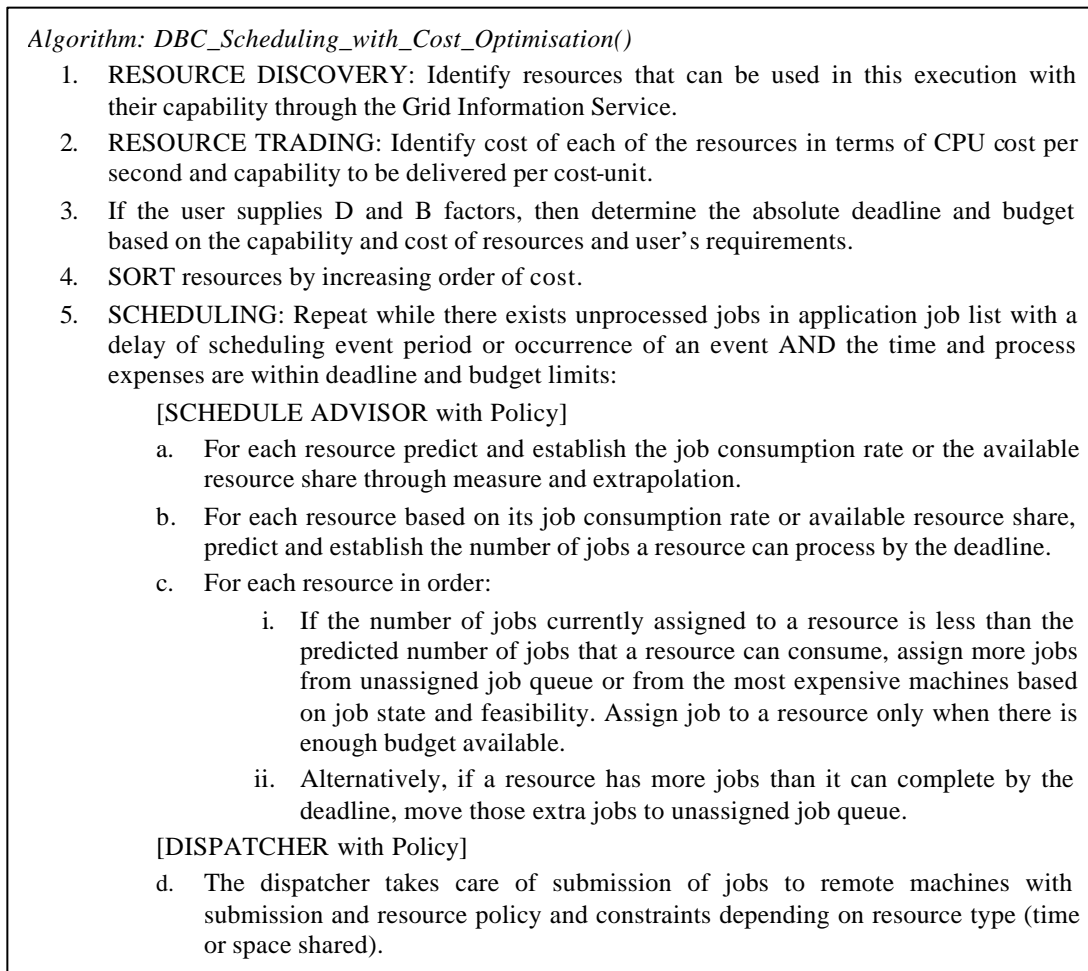
Figure 20: Deadline and budget constrained (DBC) scheduling with cost-optimization.
